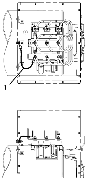
6000 SERIES ALTERNATOR
