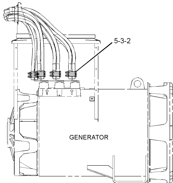
(ALTERNATOR CONNECTION)
