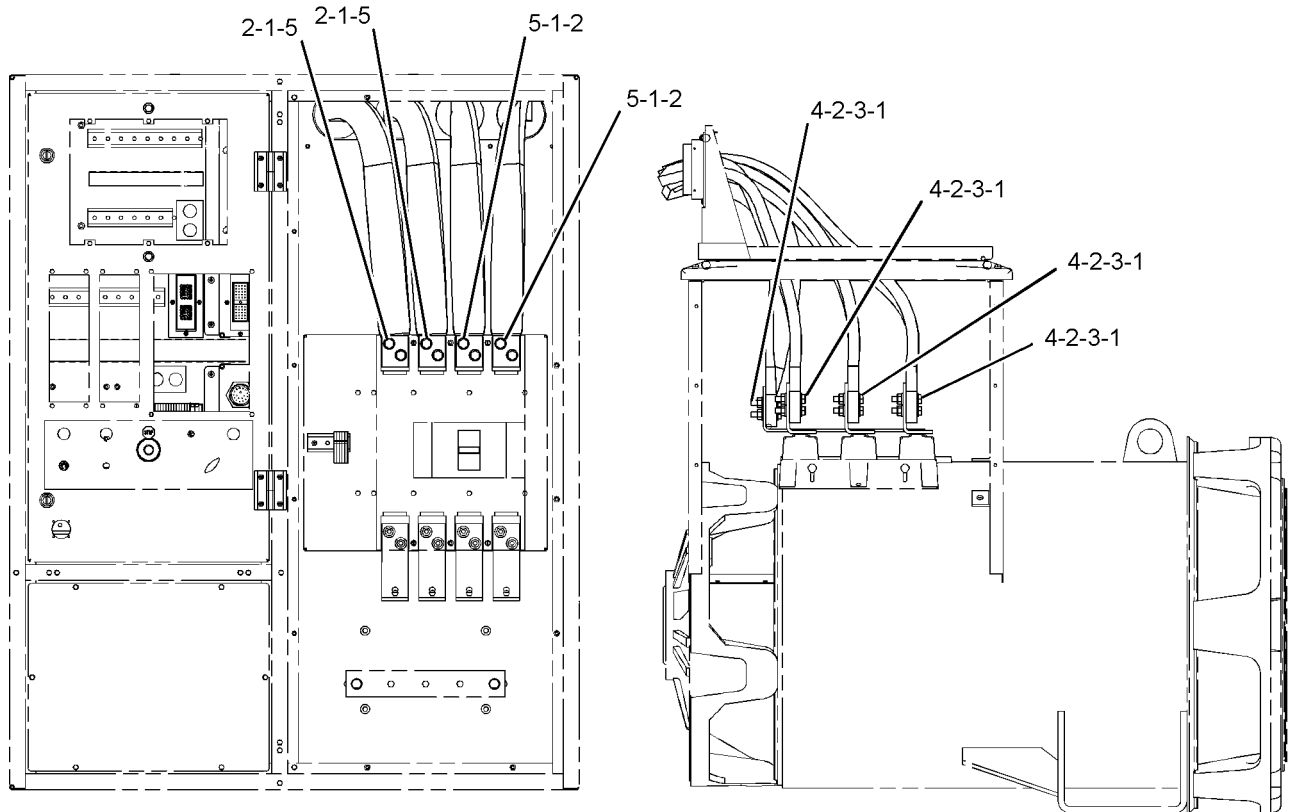
BREAKER CONNECTION
